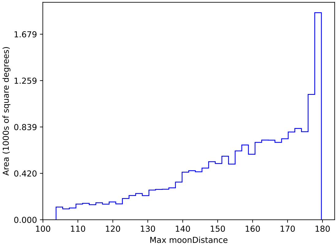
too_elab_r8_d3_griz_v3.4_10yrs WFD all bands: Max moonDistance
