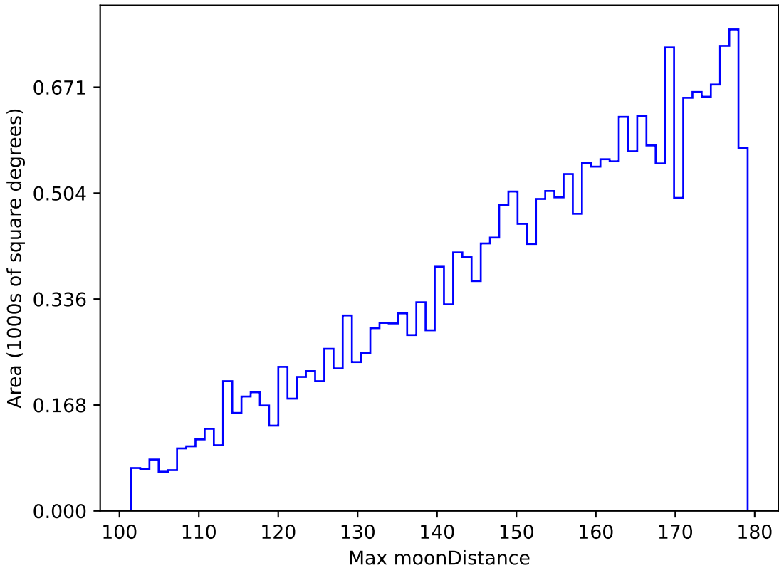
too_elab_r8_d3_griz_v3.4_10yrs All sky u band: Max moonDistance
