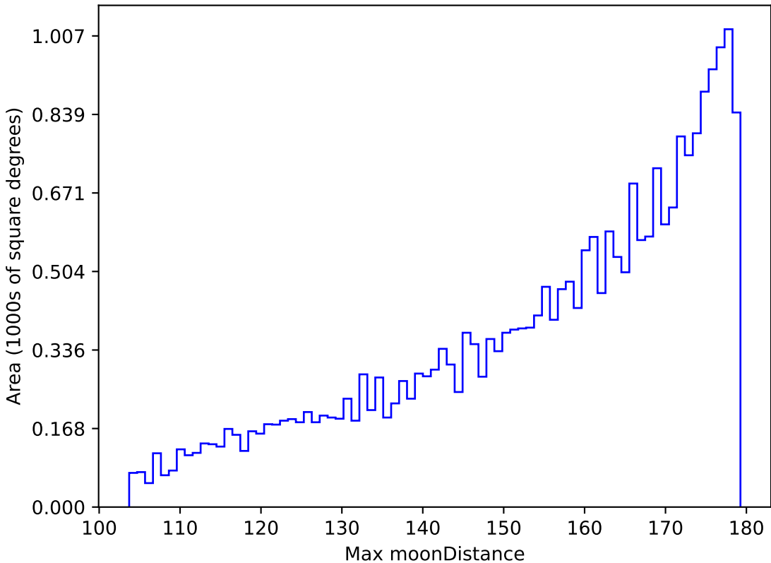
too_elab_r8_d3_griz_v3.4_10yrs All sky i band: Max moonDistance
