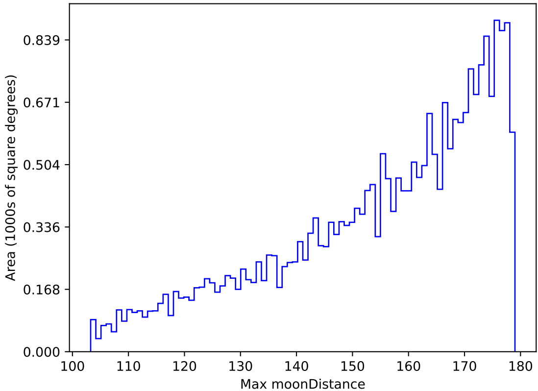
too_elab_r8_d3_griz_v3.4_10yrs All sky g band: Max moonDistance
