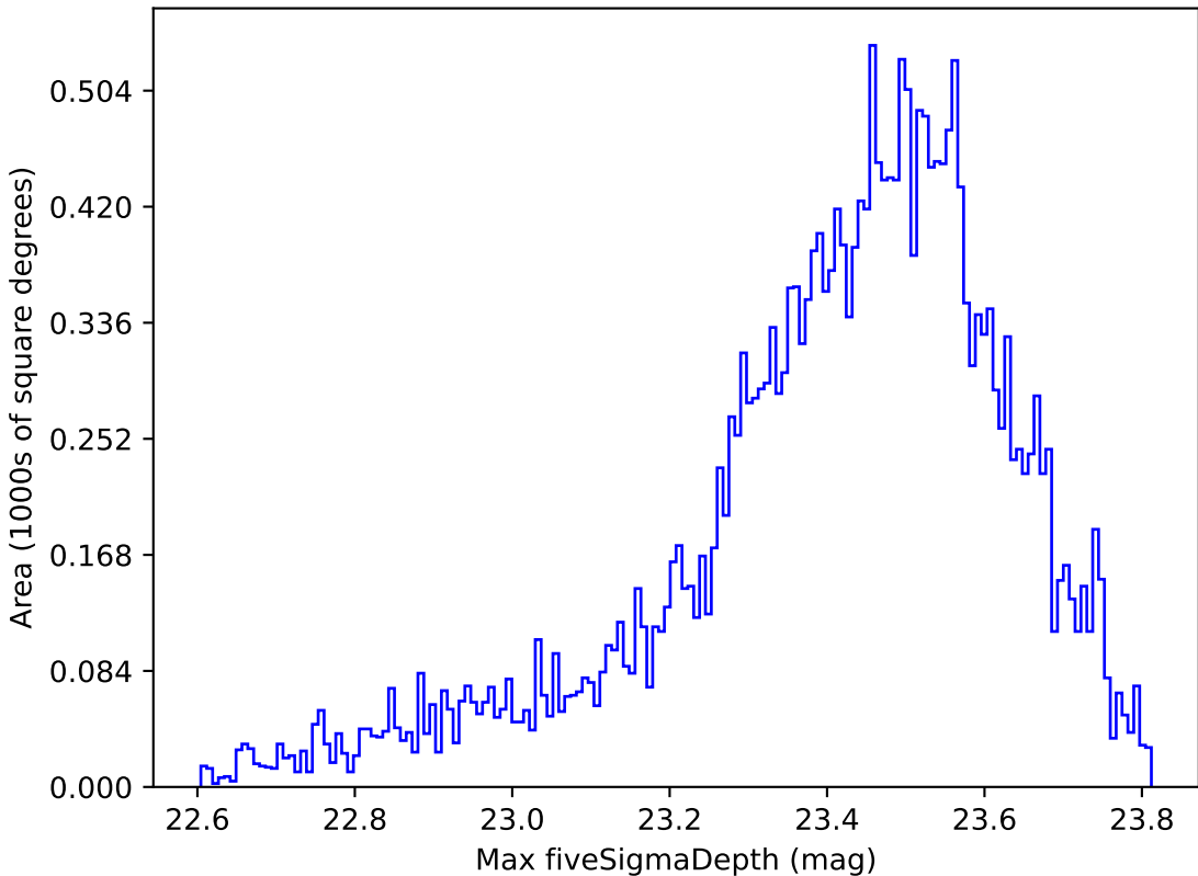
too_elab_r8_d3_griz_v3.4_10yrs Yr 1 z band: Max fiveSigmaDepth
