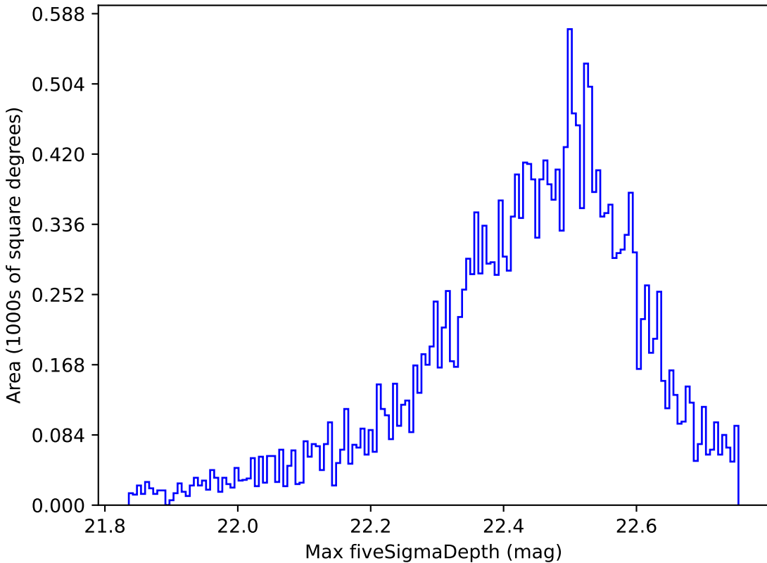
too_elab_r8_d3_griz_v3.4_10yrs Yr 1 y band: Max fiveSigmaDepth
