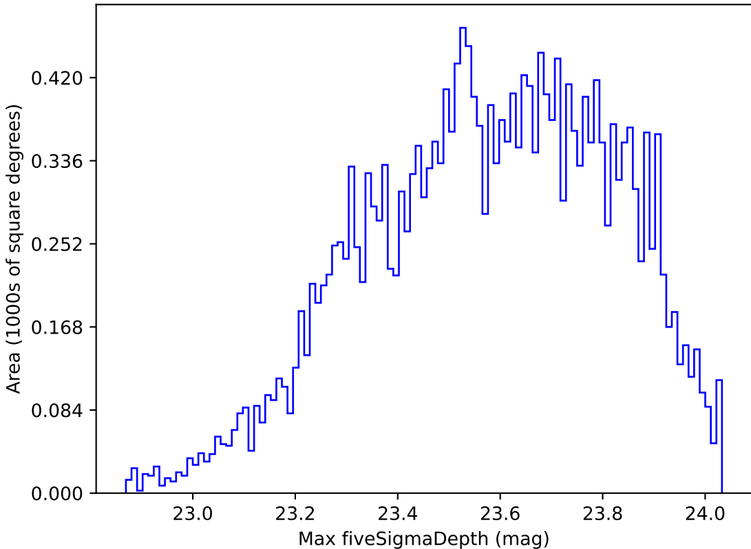
too_elab_r8_d3_griz_v3.4_10yrs Yr 1 u band: Max fiveSigmaDepth
