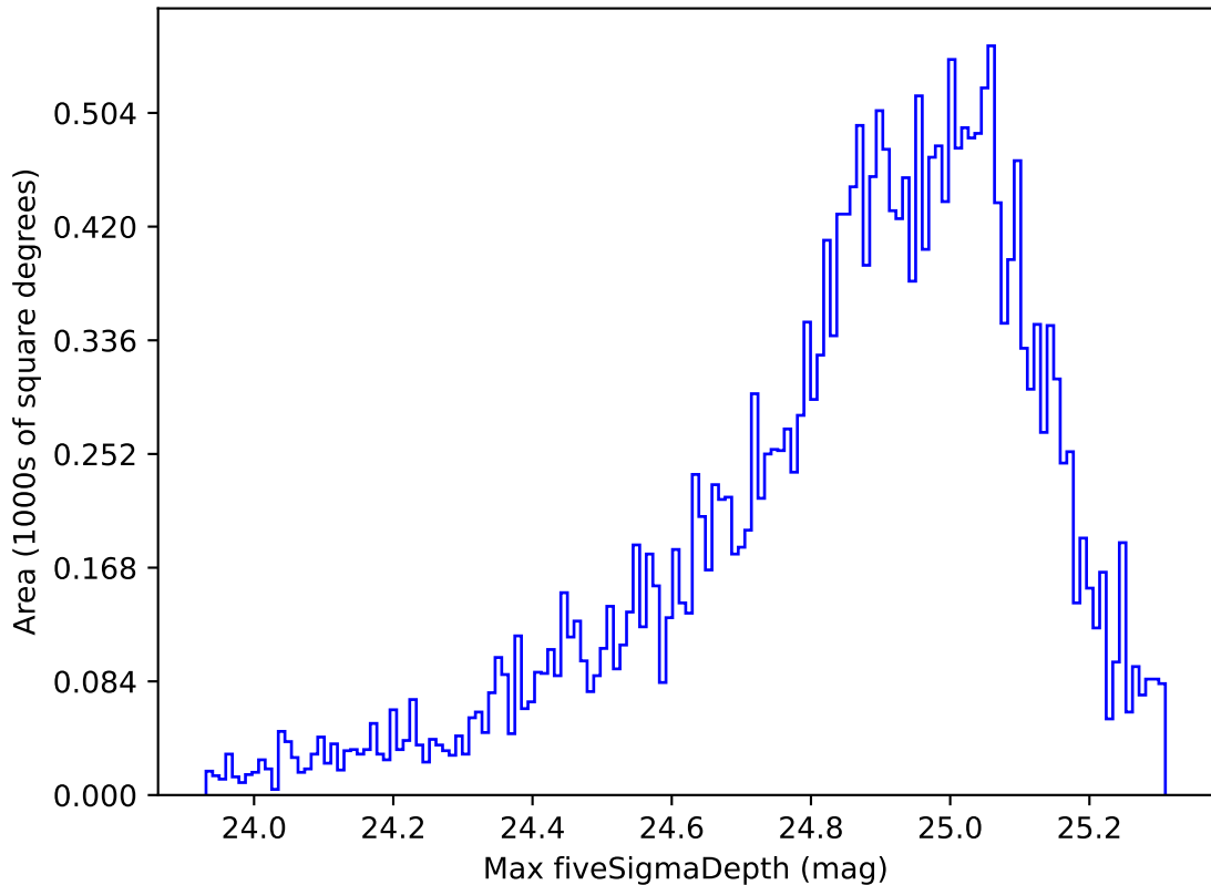
too_elab_r8_d3_griz_v3.4_10yrs Yr 1 g band: Max fiveSigmaDepth
