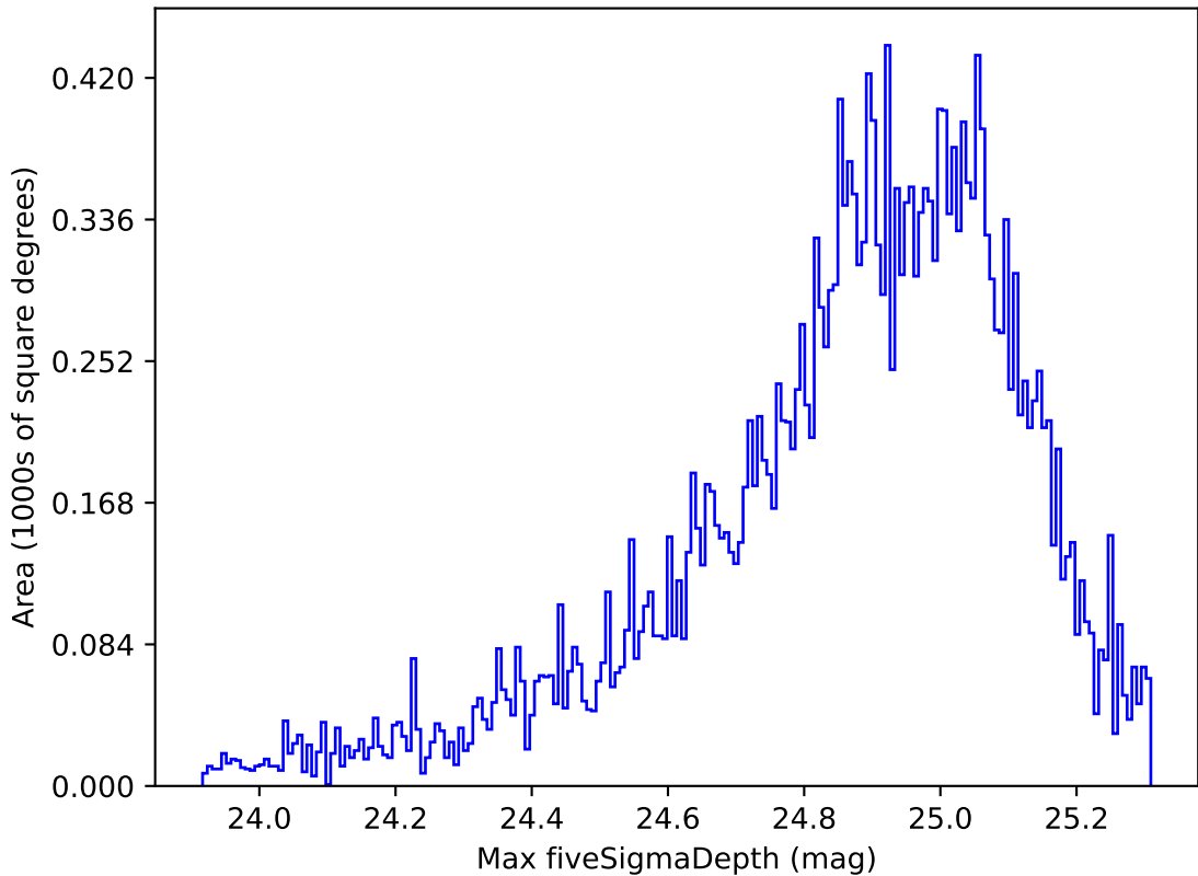
too_elab_r8_d3_griz_v3.4_10yrs Yr 1 all bands: Max fiveSigmaDepth
