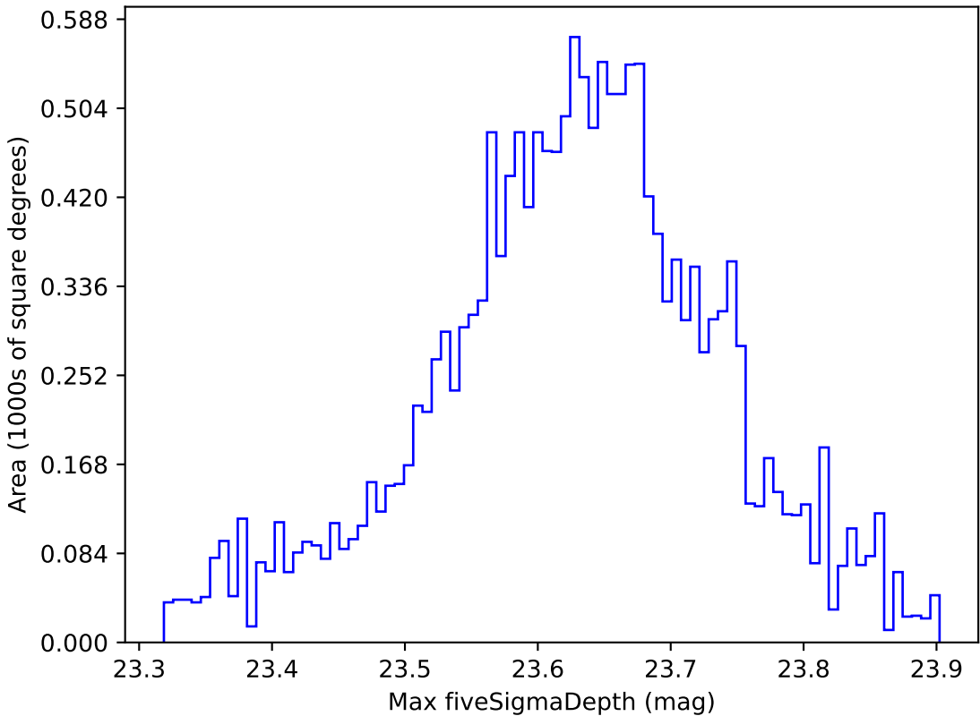
too_elab_r8_d3_griz_v3.4_10yrs WFD z band: Max fiveSigmaDepth
