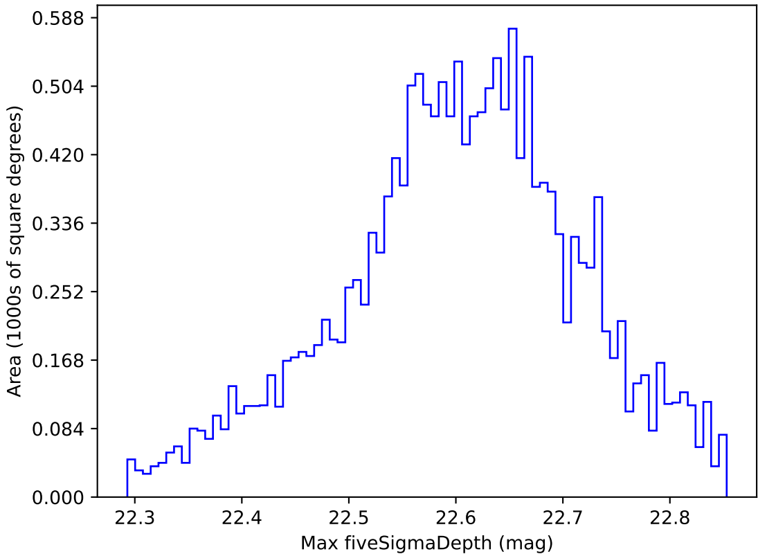
too_elab_r8_d3_griz_v3.4_10yrs WFD y band: Max fiveSigmaDepth
