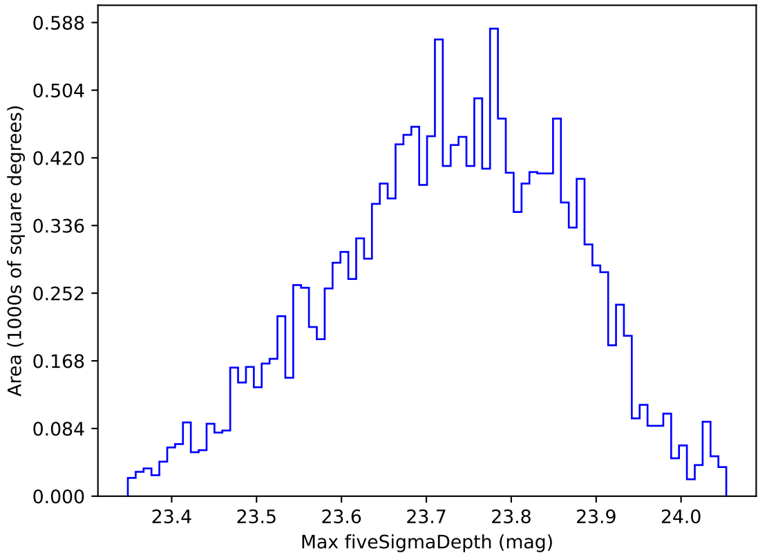
too_elab_r8_d3_griz_v3.4_10yrs WFD u band: Max fiveSigmaDepth
