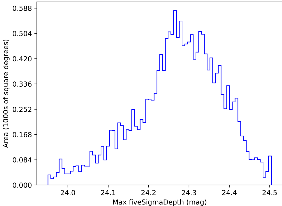
too_elab_r8_d3_griz_v3.4_10yrs WFD i band: Max fiveSigmaDepth
