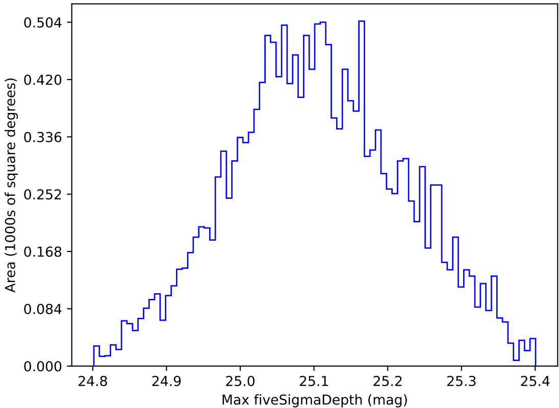
too_elab_r8_d3_griz_v3.4_10yrs WFD g band: Max fiveSigmaDepth
