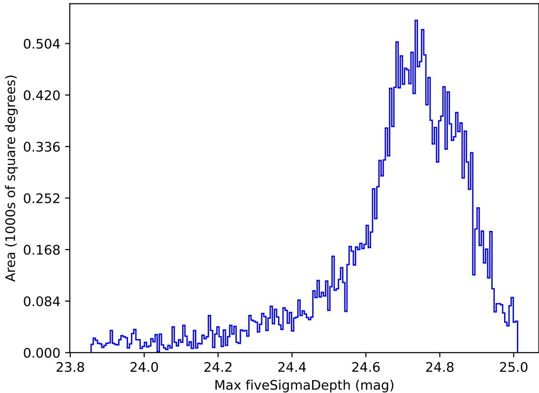
too_elab_r8_d3_griz_v3.4_10yrs All sky r band: Max fiveSigmaDepth
