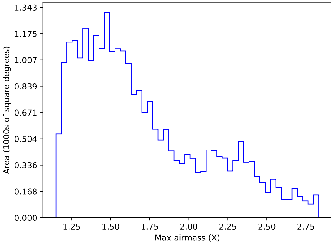
too_elab_r8_d3_griz_v3.4_10yrs Yr 1 z band: Max airmass
