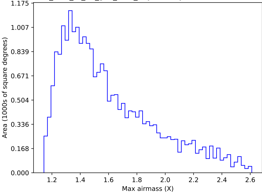
too_elab_r8_d3_griz_v3.4_10yrs Yr 1 y band: Max airmass
