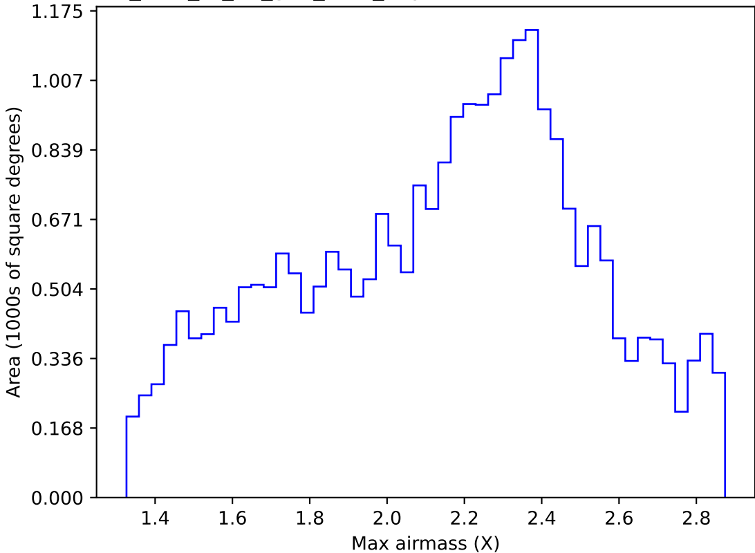
too_elab_r8_d3_griz_v3.4_10yrs Yr 1 all bands: Max airmass
