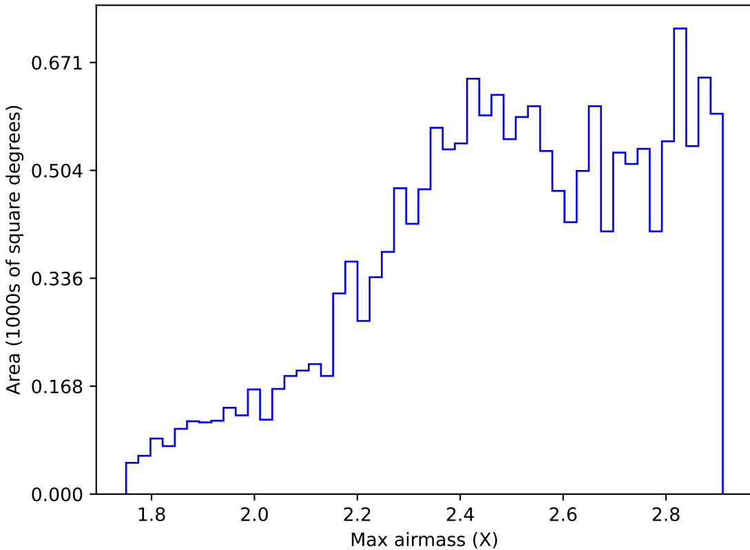
too_elab_r8_d3_griz_v3.4_10yrs WFD z band: Max airmass
