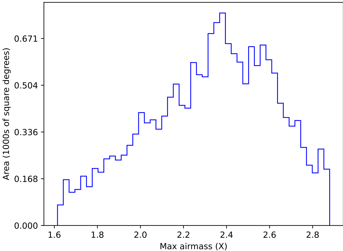
too_elab_r8_d3_griz_v3.4_10yrs WFD y band: Max airmass
