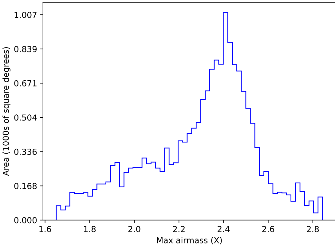
too_elab_r8_d3_griz_v3.4_10yrs WFD r band: Max airmass
