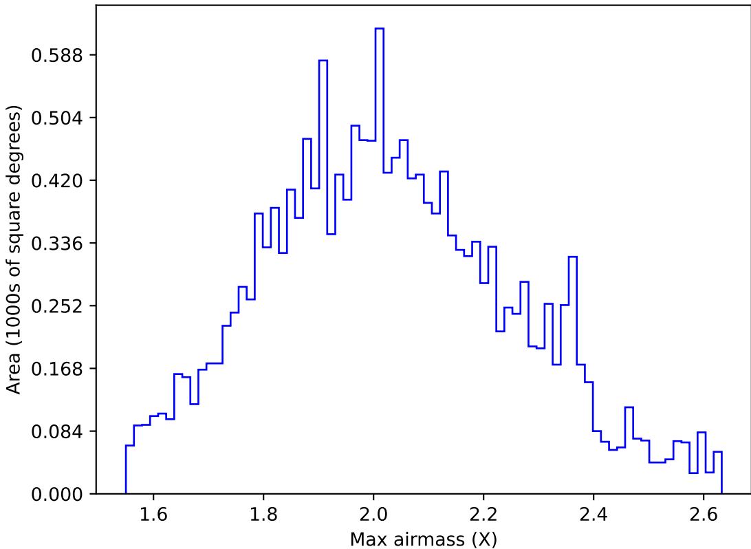
too_elab_r8_d3_griz_v3.4_10yrs WFD g band: Max airmass
