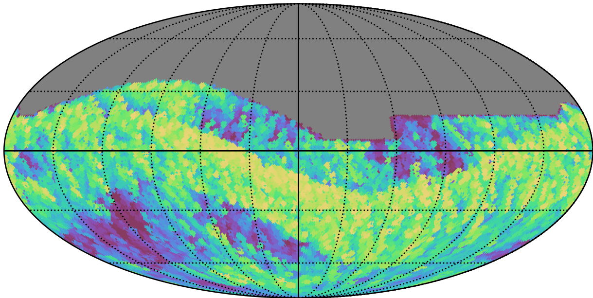
too_elab_r8_d3_griz_v3.4_10yrs All sky z band: Max airmass
