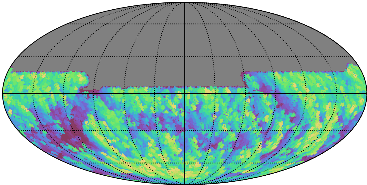
too_elab_r8_d3_griz_v3.4_10yrs All sky y band: Max airmass
