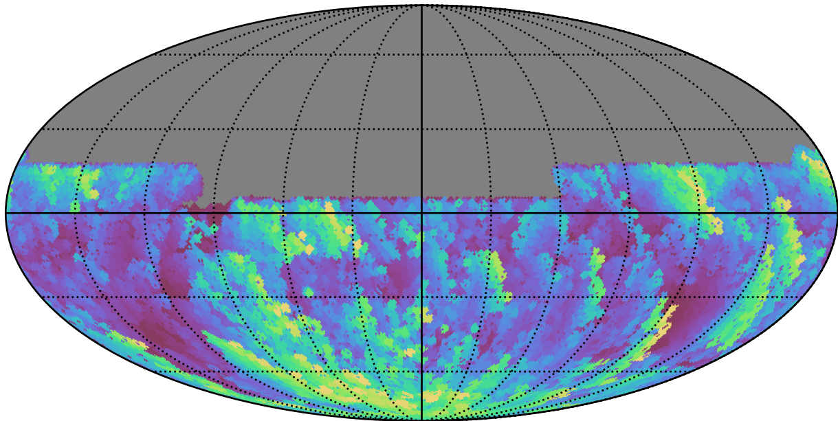
too_elab_r8_d3_griz_v3.4_10yrs All sky u band: Max airmass
