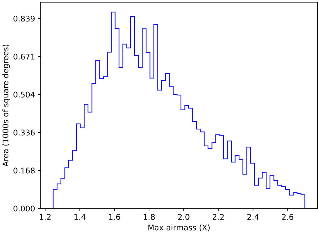
too_elab_r8_d3_griz_v3.4_10yrs All sky u band: Max airmass
