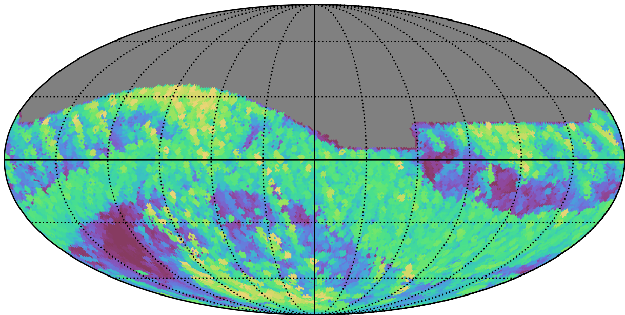
too_elab_r8_d3_griz_v3.4_10yrs All sky r band: Max airmass
