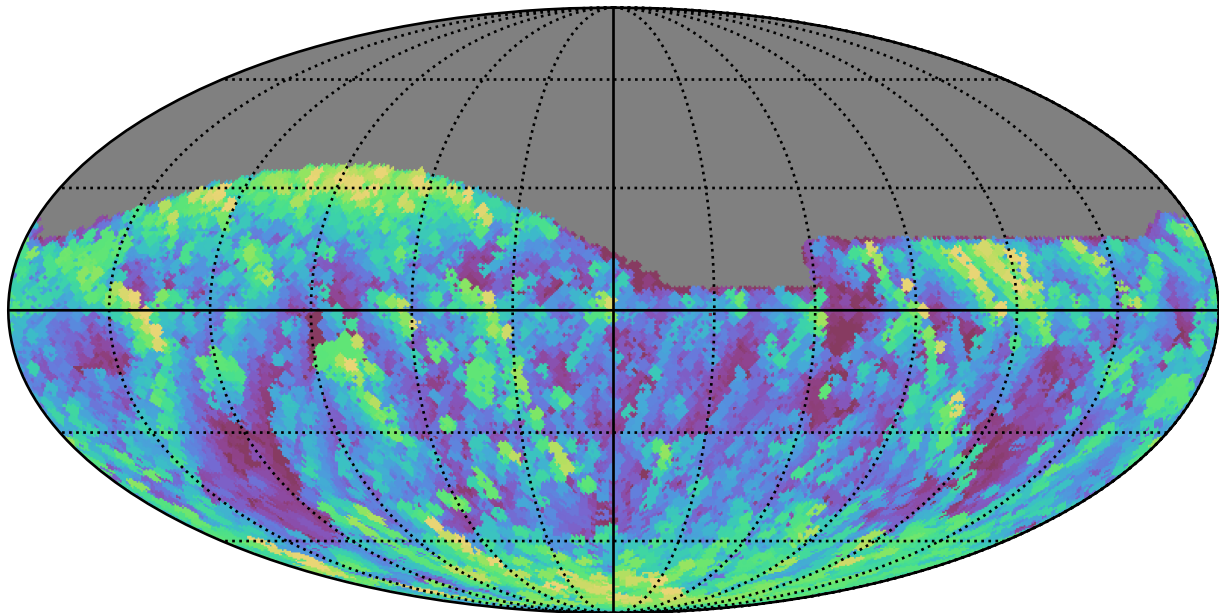
too_elab_r8_d3_griz_v3.4_10yrs All sky g band: Max airmass
