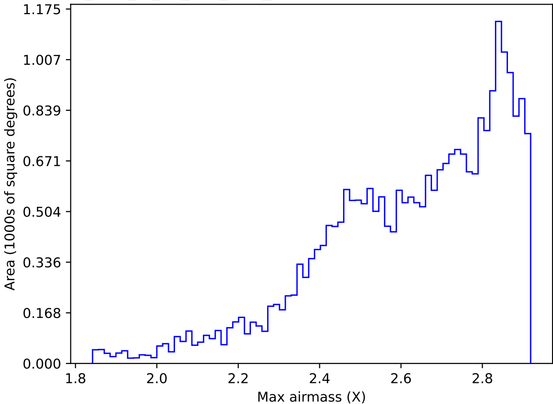
too_elab_r8_d3_griz_v3.4_10yrs All sky all bands: Max airmass
