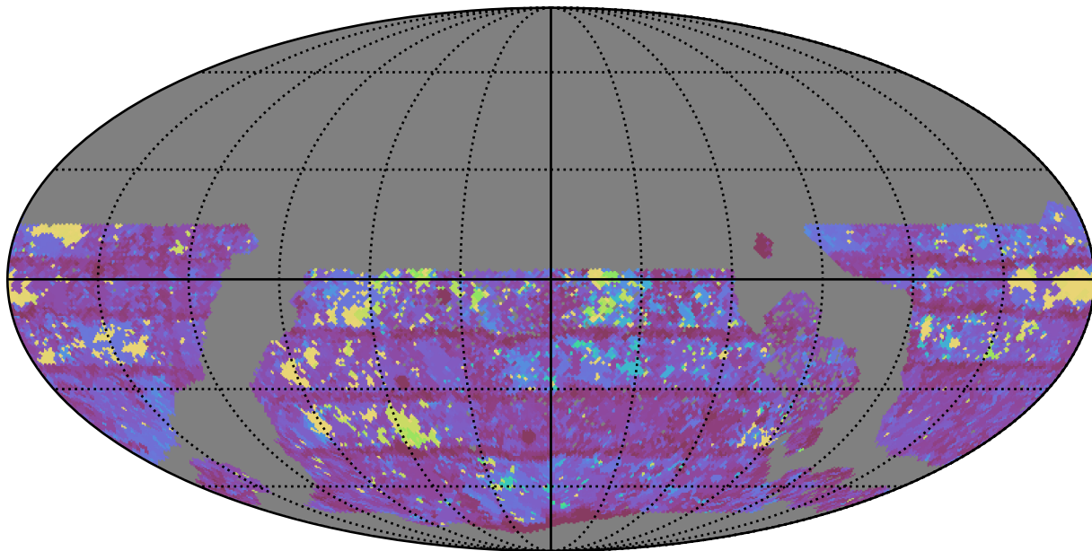
too_elab_r8_d3_griz_v3.4_10yrs WFD y band: Max Inter-Night Gap
