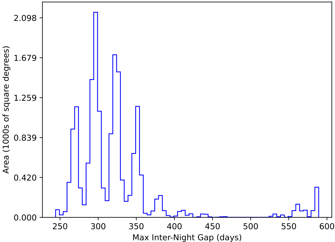
too_elab_r8_d3_griz_v3.4_10yrs WFD y band: Max Inter-Night Gap
