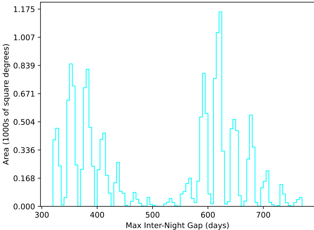
too_elab_r8_d3_griz_v3.4_10yrs WFD u band: Max Inter-Night Gap
