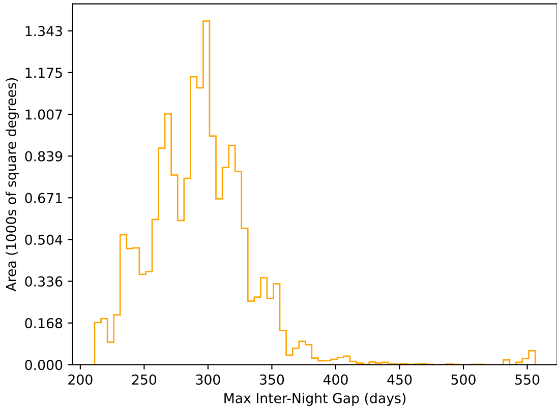
too_elab_r8_d3_griz_v3.4_10yrs WFD r band: Max Inter-Night Gap
