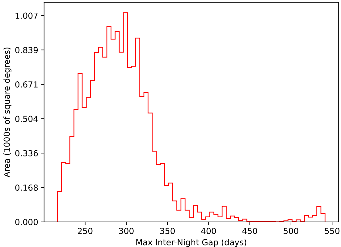
too_elab_r8_d3_griz_v3.4_10yrs WFD i band: Max Inter-Night Gap
