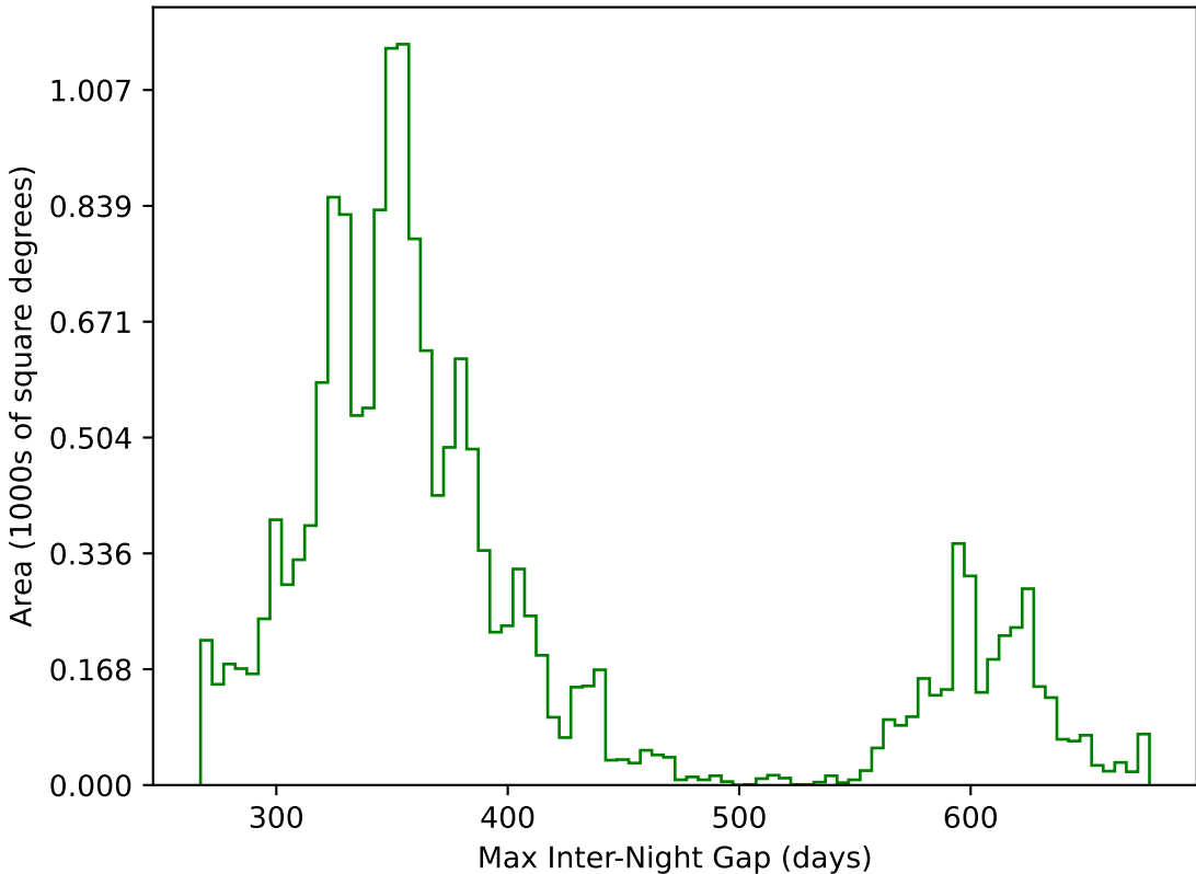
too_elab_r8_d3_griz_v3.4_10yrs WFD g band: Max Inter-Night Gap
