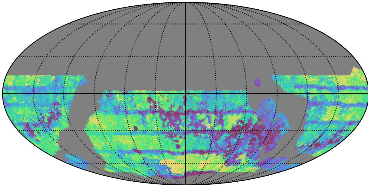
too_elab_r8_d3_griz_v3.4_10yrs WFD all bands: Max Inter-Night Gap
