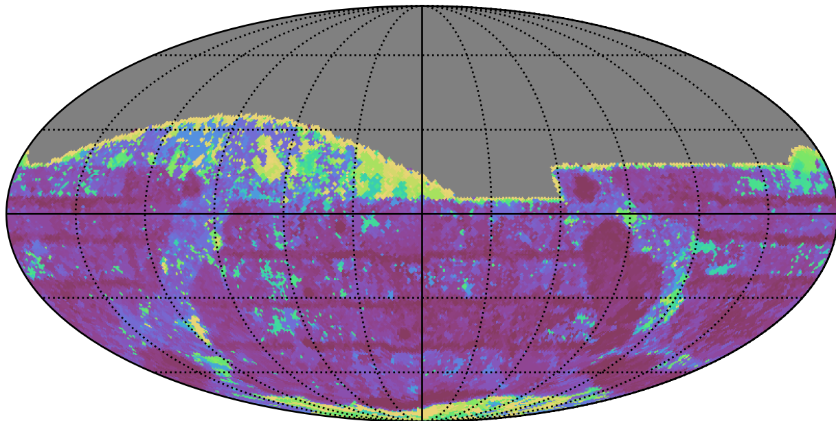
too_elab_r8_d3_griz_v3.4_10yrs All sky z band: Max Inter-Night Gap
