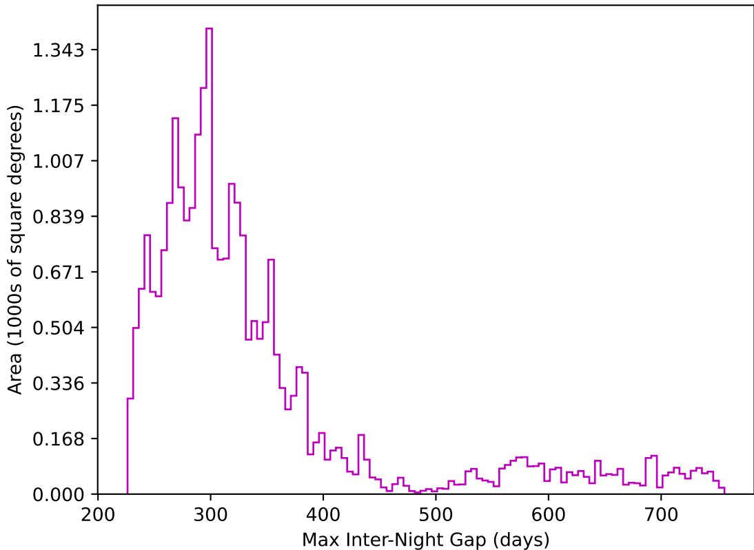
too_elab_r8_d3_griz_v3.4_10yrs All sky z band: Max Inter-Night Gap
