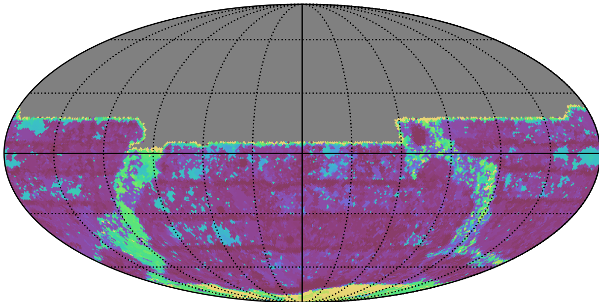
too_elab_r8_d3_griz_v3.4_10yrs All sky y band: Max Inter-Night Gap
