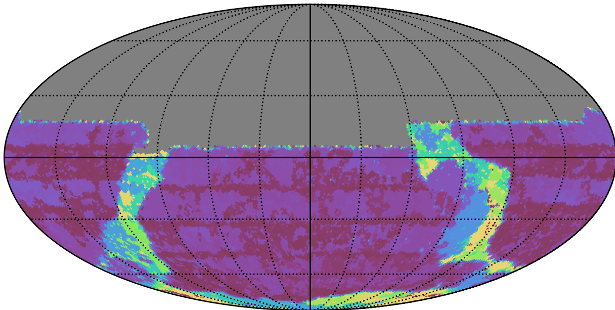
too_elab_r8_d3_griz_v3.4_10yrs All sky u band: Max Inter-Night Gap
