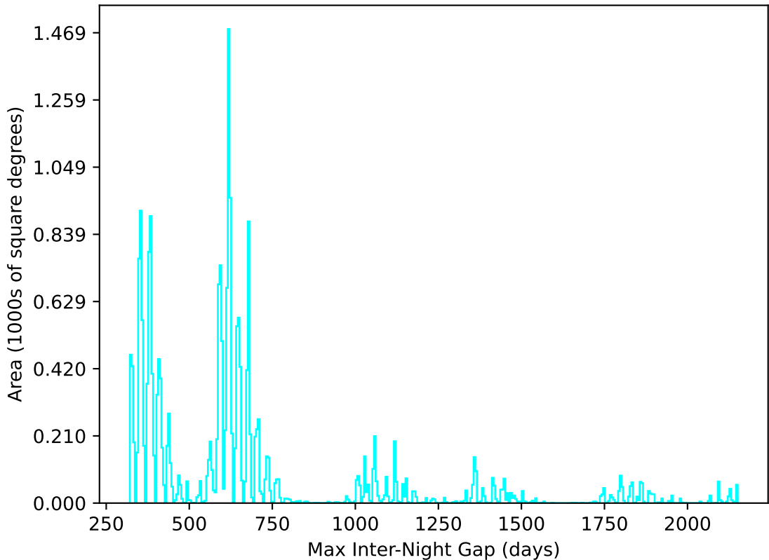
too_elab_r8_d3_griz_v3.4_10yrs All sky u band: Max Inter-Night Gap
