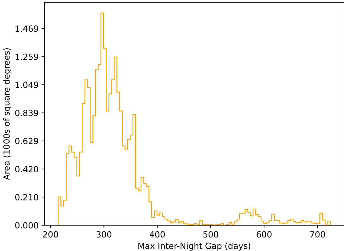
too_elab_r8_d3_griz_v3.4_10yrs All sky r band: Max Inter-Night Gap
