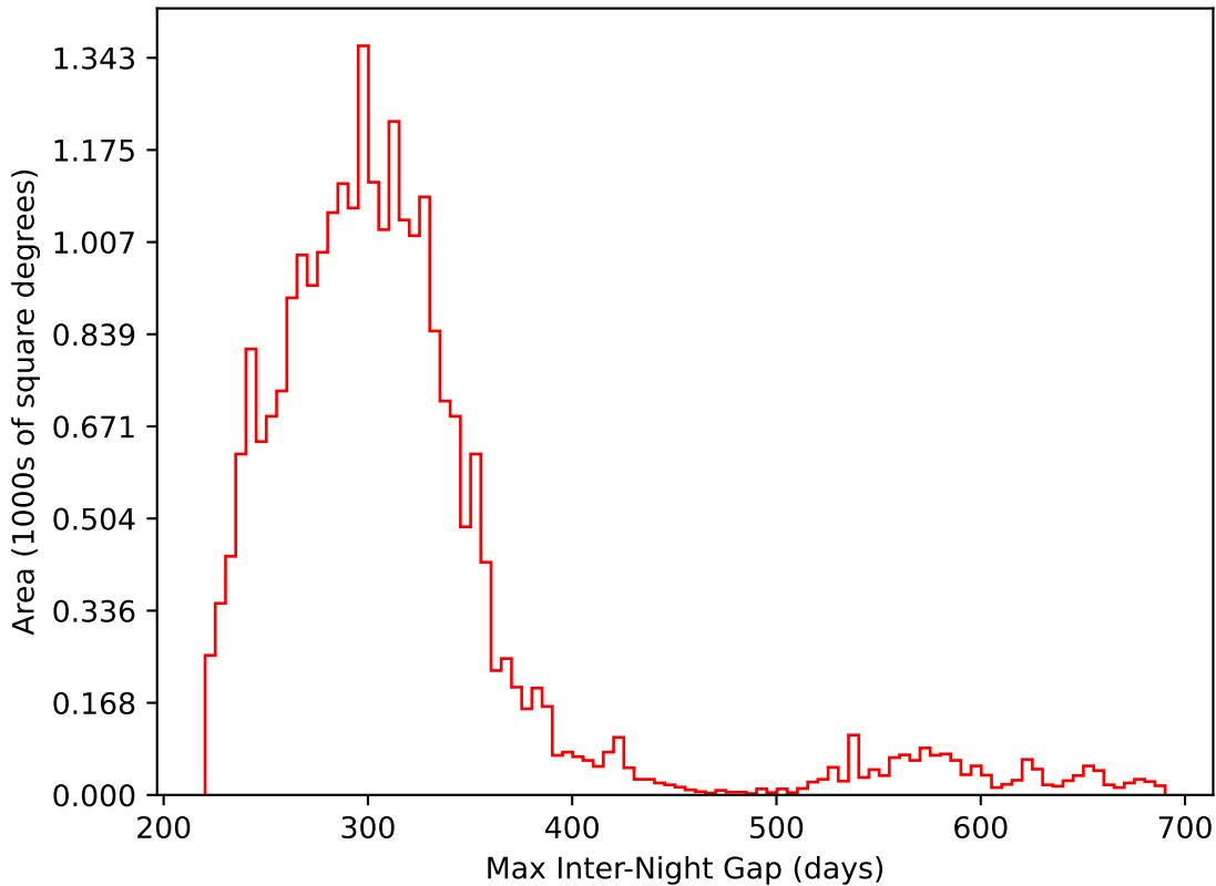
too_elab_r8_d3_griz_v3.4_10yrs All sky i band: Max Inter-Night Gap
