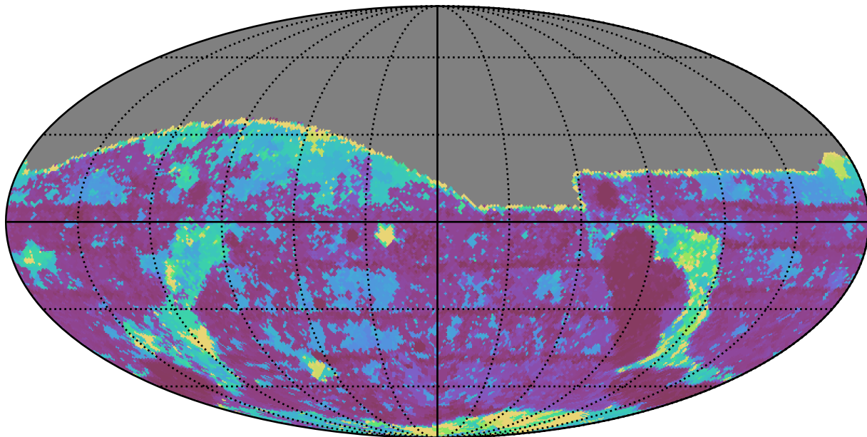
too_elab_r8_d3_griz_v3.4_10yrs All sky g band: Max Inter-Night Gap
