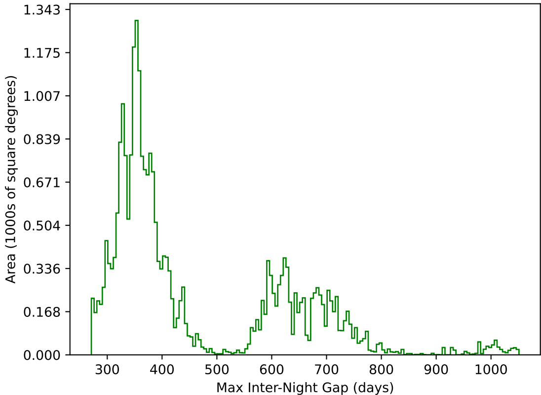
too_elab_r8_d3_griz_v3.4_10yrs All sky g band: Max Inter-Night Gap
