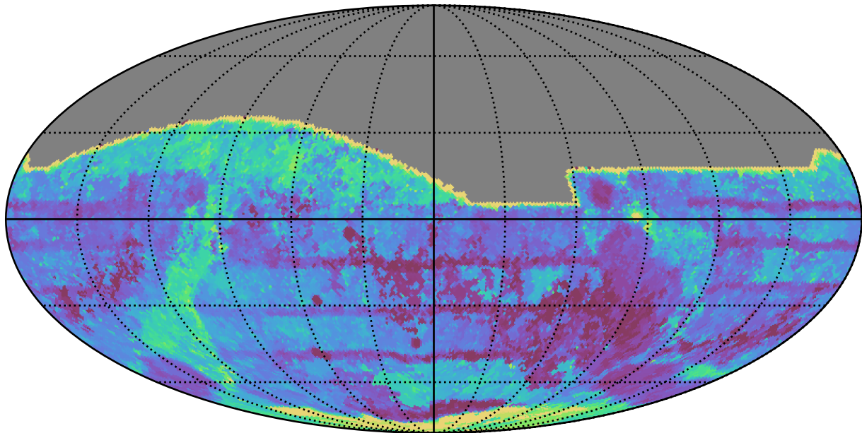
too_elab_r8_d3_griz_v3.4_10yrs All sky all bands: Max Inter-Night Gap
