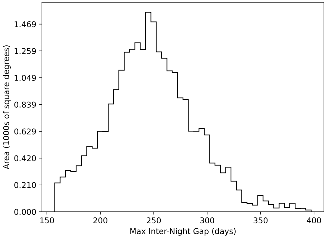
too_elab_r8_d3_griz_v3.4_10yrs All sky all bands: Max Inter-Night Gap
