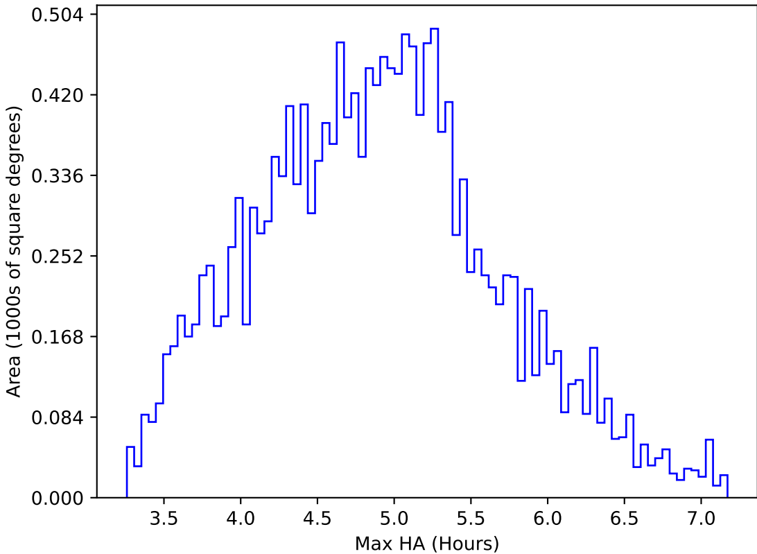
too_elab_r8_d3_griz_v3.4_10yrs WFD z band: Max HA
