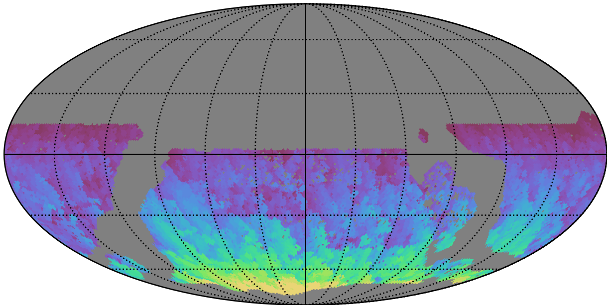
too_elab_r8_d3_griz_v3.4_10yrs WFD y band: Max HA
