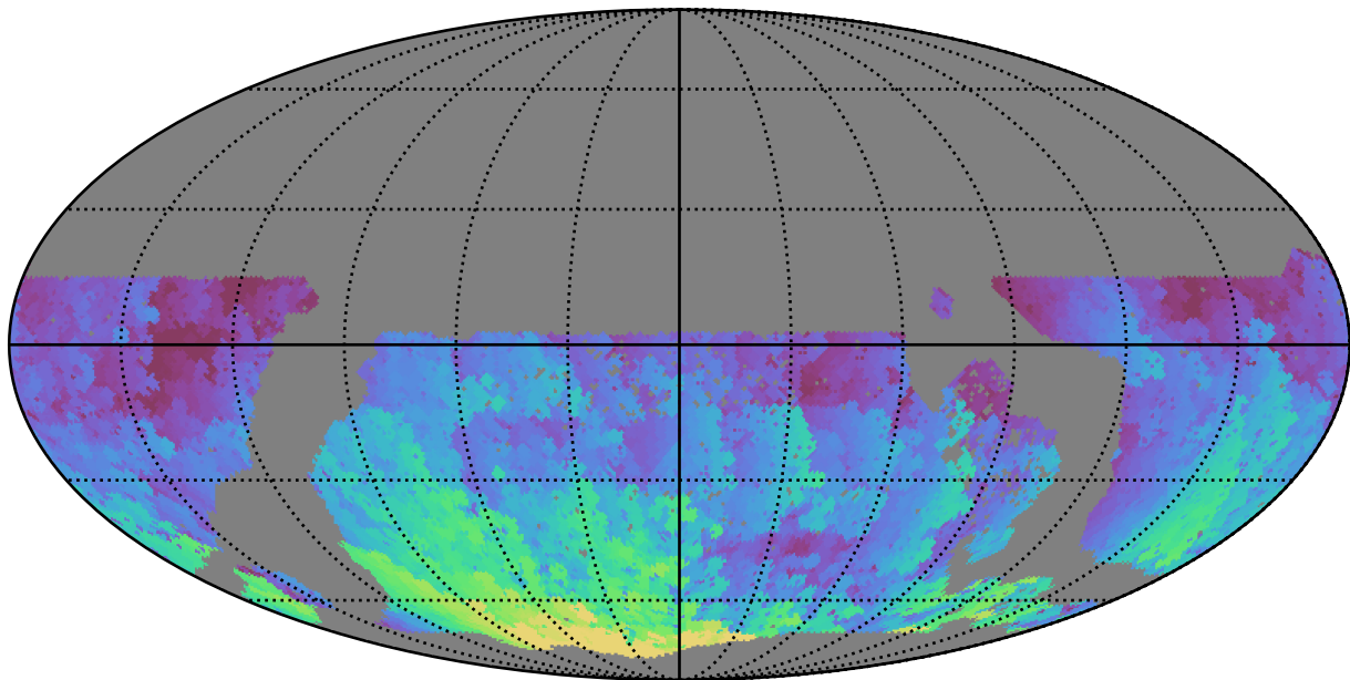
too_elab_r8_d3_griz_v3.4_10yrs WFD u band: Max HA
